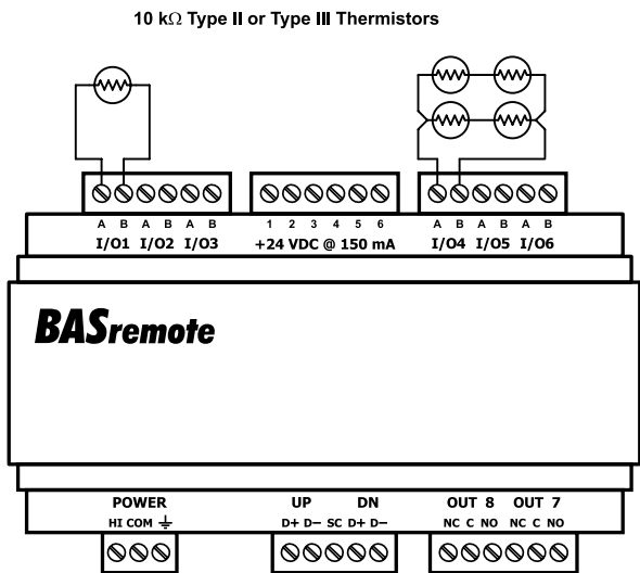
Figure 11 — Thermistor Connections
