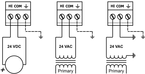
Figure 8 — Power Options
